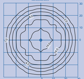
400W MH @ 20' Mounting Height Isofootcandles
